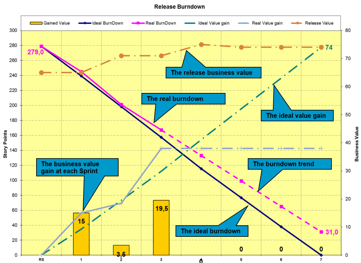
Figure 4: Example of Release Burndown Chart
